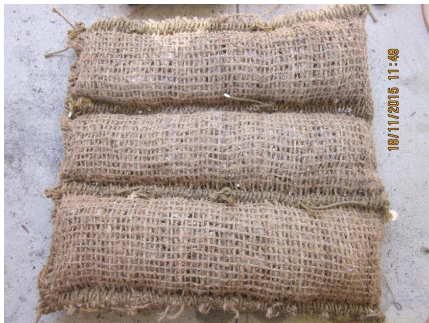
Figure 5-3: Example Triple Oyster Shell Filled Bag
